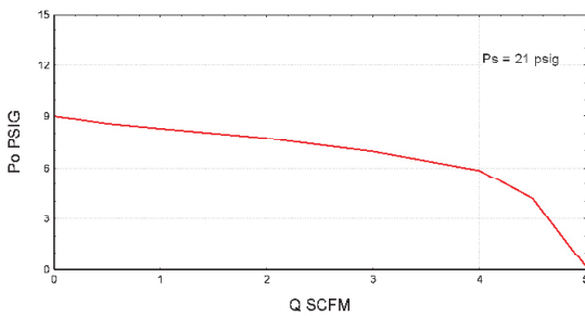
T6100 Transducer Flow Characteristics
